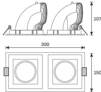
Cut-Out: 290 x 136mm *All dimensions are in mm.
